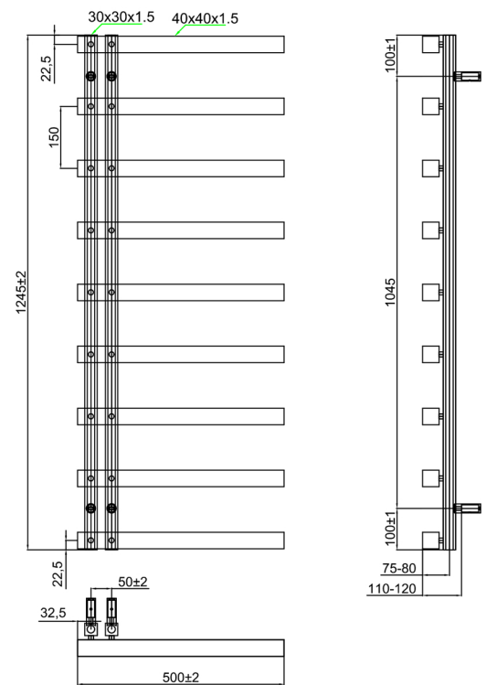
1245X500MM
