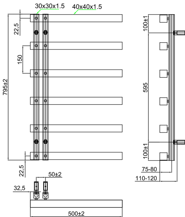
795X500MM
